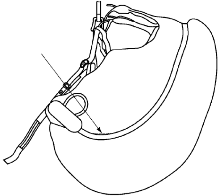
Figure 4 — Harness lower measuring point
