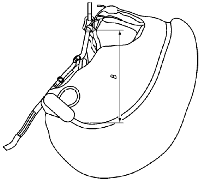
Figure 6 — Height of harness attachment points
